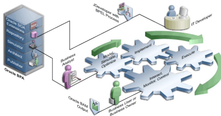
Abb. 2: BPA Round-Tripping
