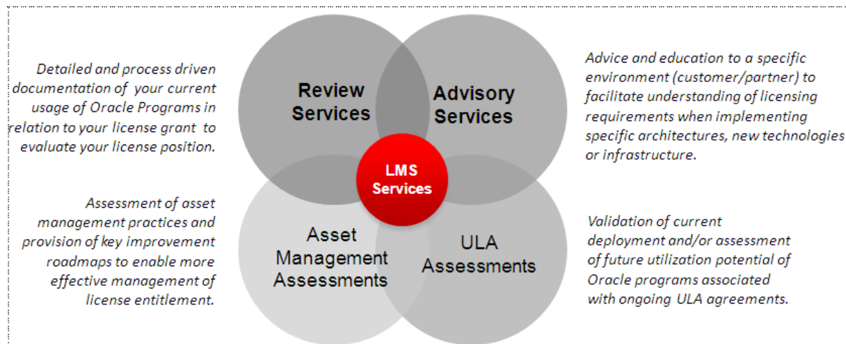
Abb. 1: LMS Services
