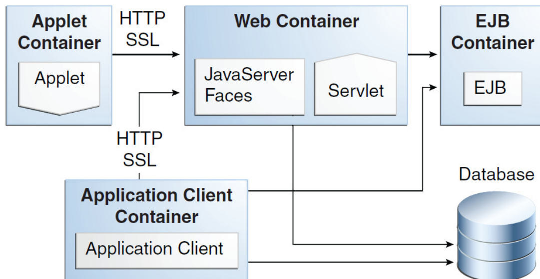
Abbildung 2: Java EE 6 API's
